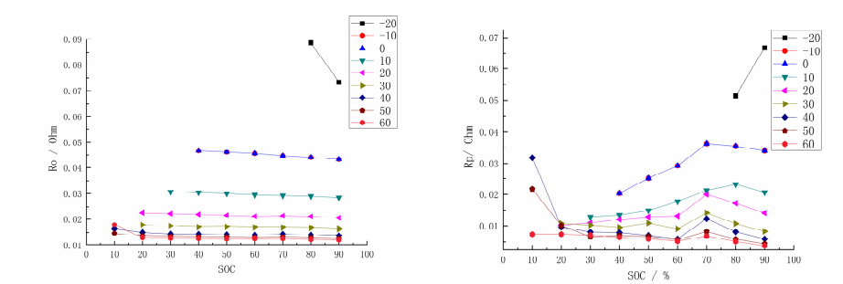
Fig. 5. The cell ohmic resistance and polarization resistance at different temperatures and SOC
