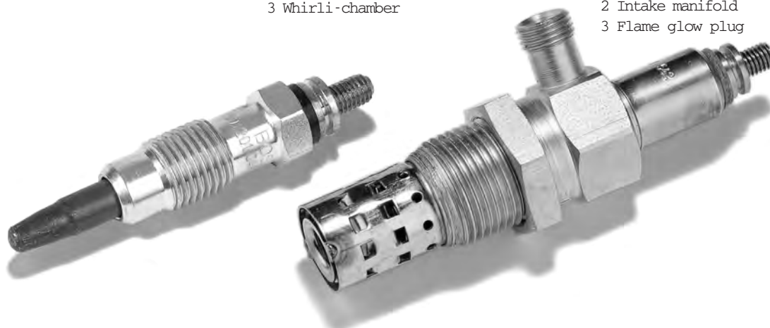
4 Starting assistance with flame glow
