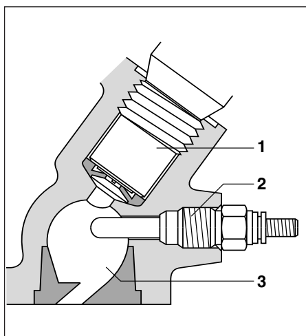
3 Whirl-chamber engine
