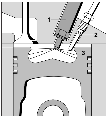
1 Direct-Injection (DI) engine
