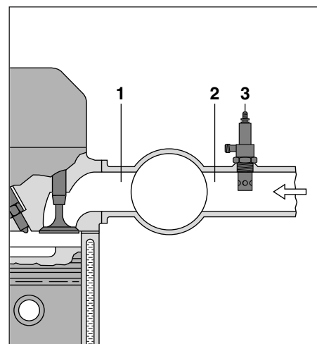
4 Starting assistance with flame glow
