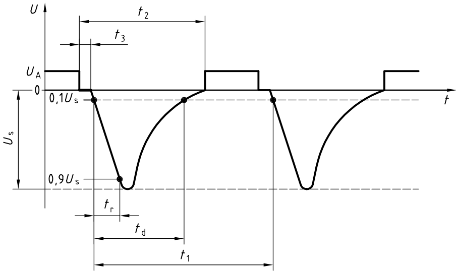
Figure 5 — Test pulse 1
