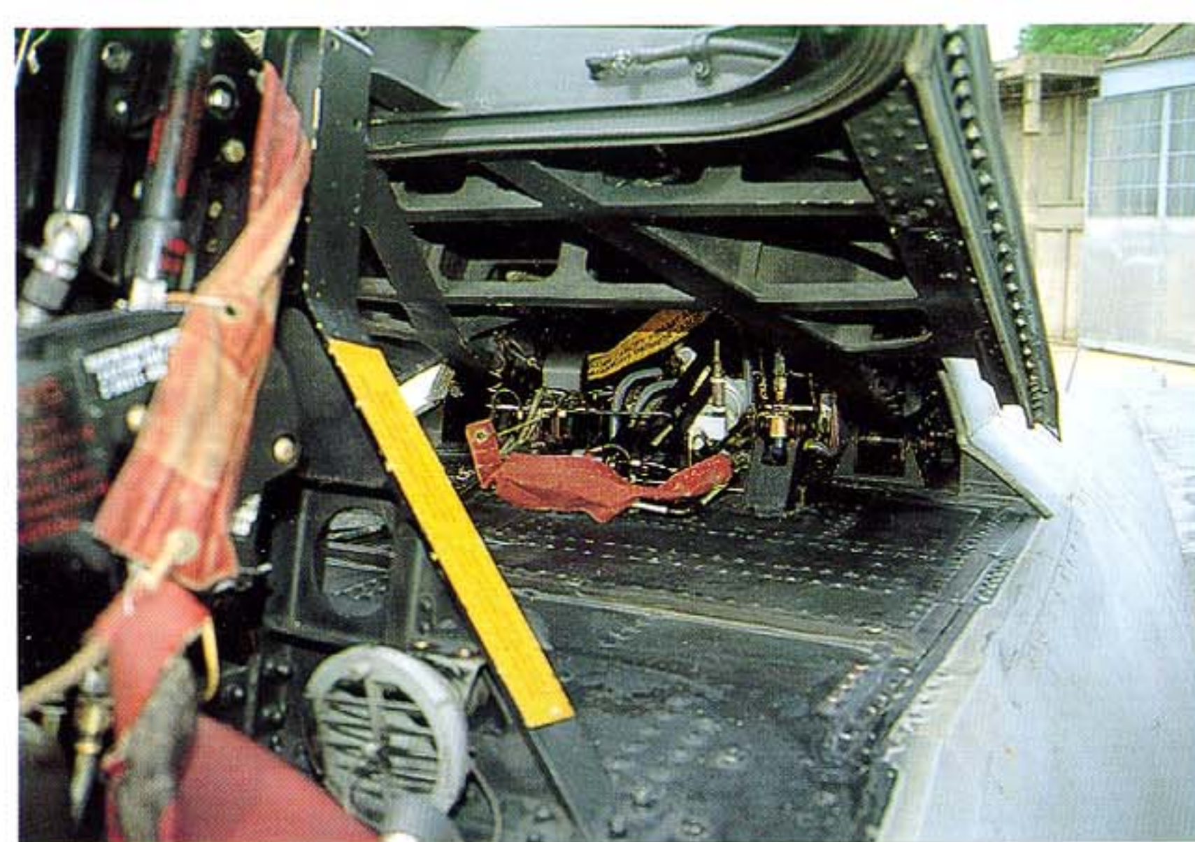
Canopy actuating mechanism at the extreme aft end of the hood. Note the solid structure of the latter.
