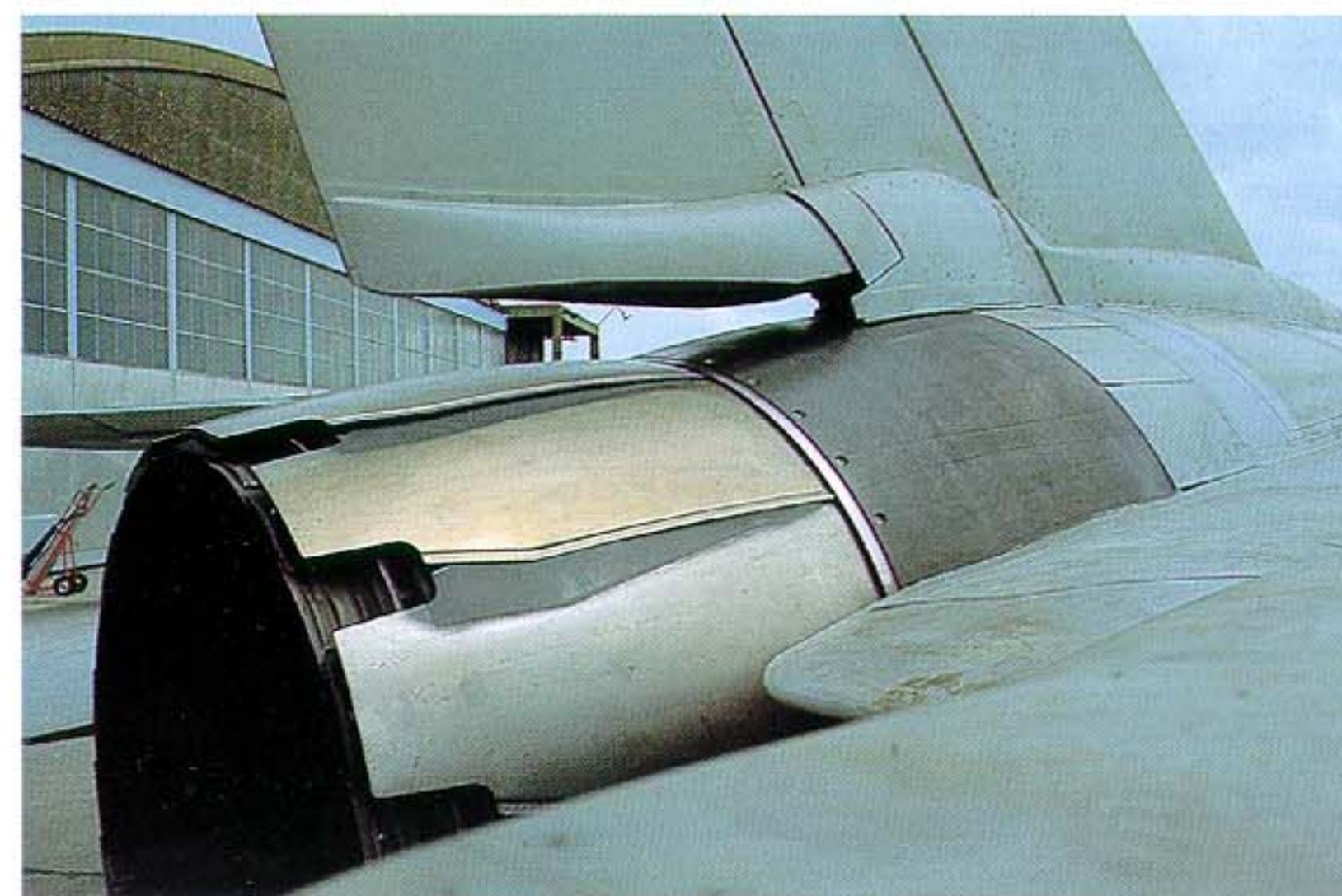
The twin vertical fins feature conventional rudders which are activated by actuators in the base of the fin, requiring complex fairings for coverage. Note the antenna housing next to the fuel dump.
