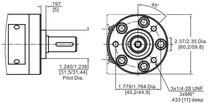
Three Bolts Mount
