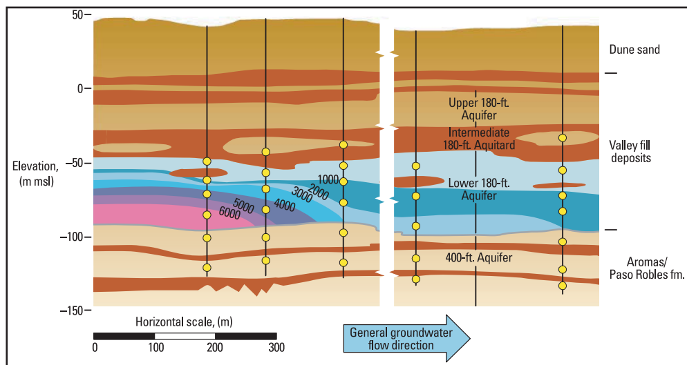
Cross-section from Fort Ord, California, shows the chloride concentration (mg/L) (after Taraszi et al., 2002).
