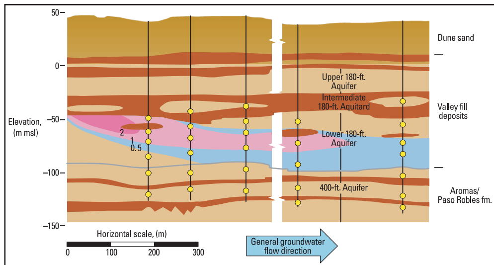
Cross-section from Fort Ord, California, shows the carbon tetrachloride concentration (µg/L) (after Taraszi et al., 2002).
